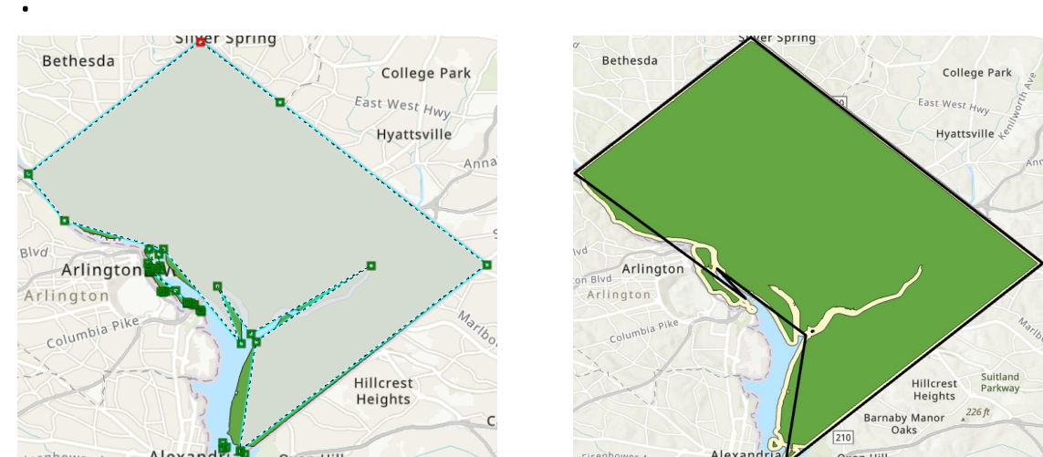
Douglas-Peucker Polygon Simplification (Retain Critical Points) in ArcPro: Simplifies to 53 vertices
