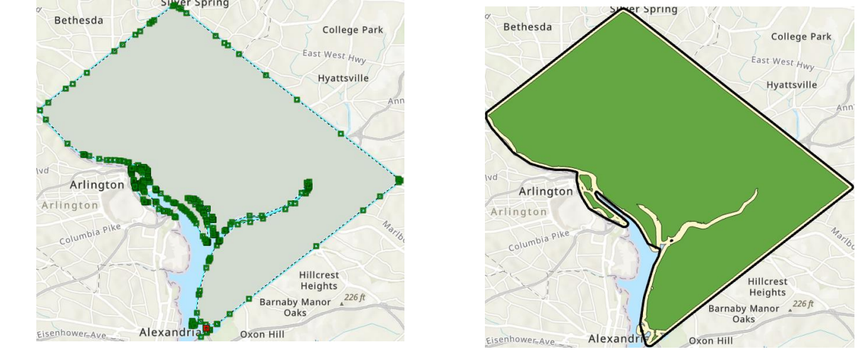
Wang-Mueller Polygon Simplification (Retain Critical Bends) in ArcPro: Simplifies to 418 vertices
