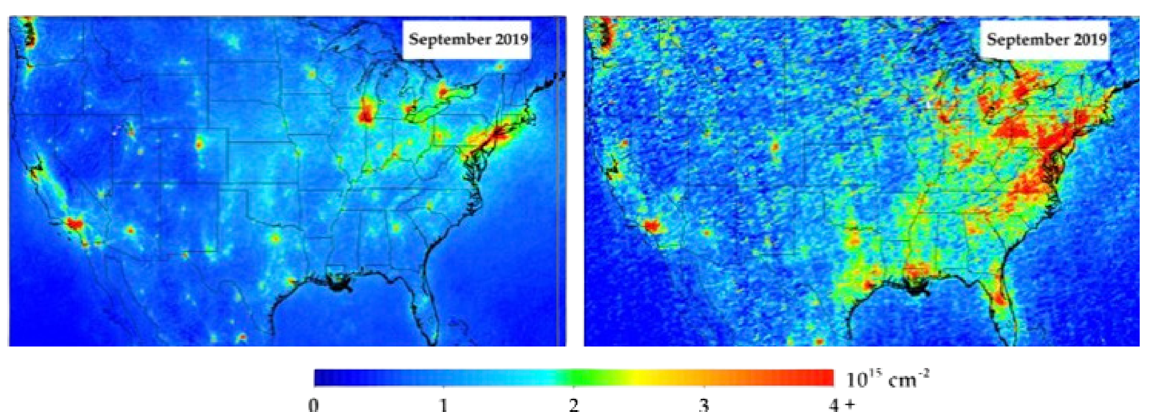
Column NO 2 as measured by OMI (left) and TROPOMI (right) satellites. Satellite images presented by Dan Goldberg.
